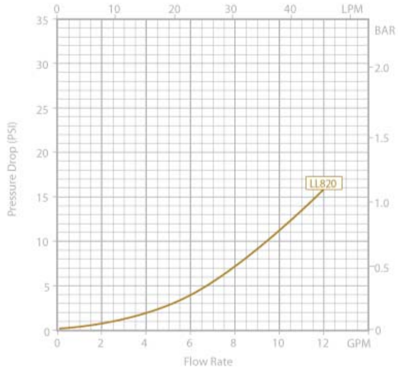
Pressure Drop Using Water
