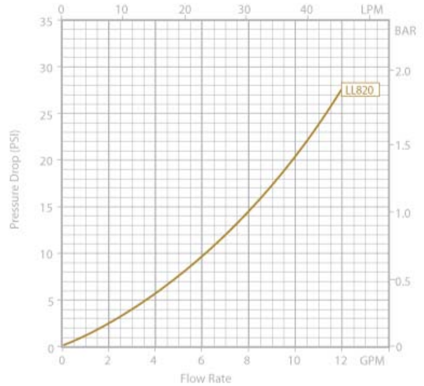
Pressure Drop Using Oil
