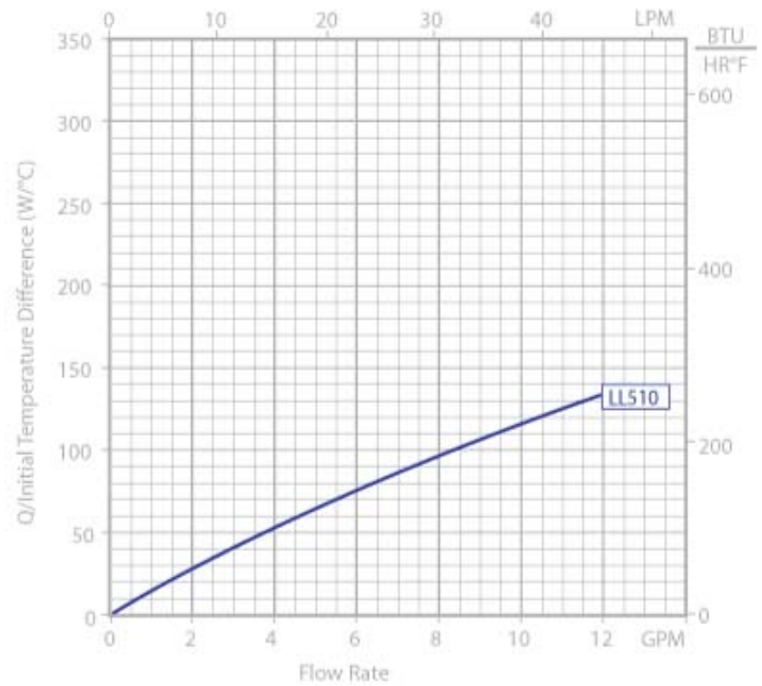
Thermal Performance Using Water and Oil
