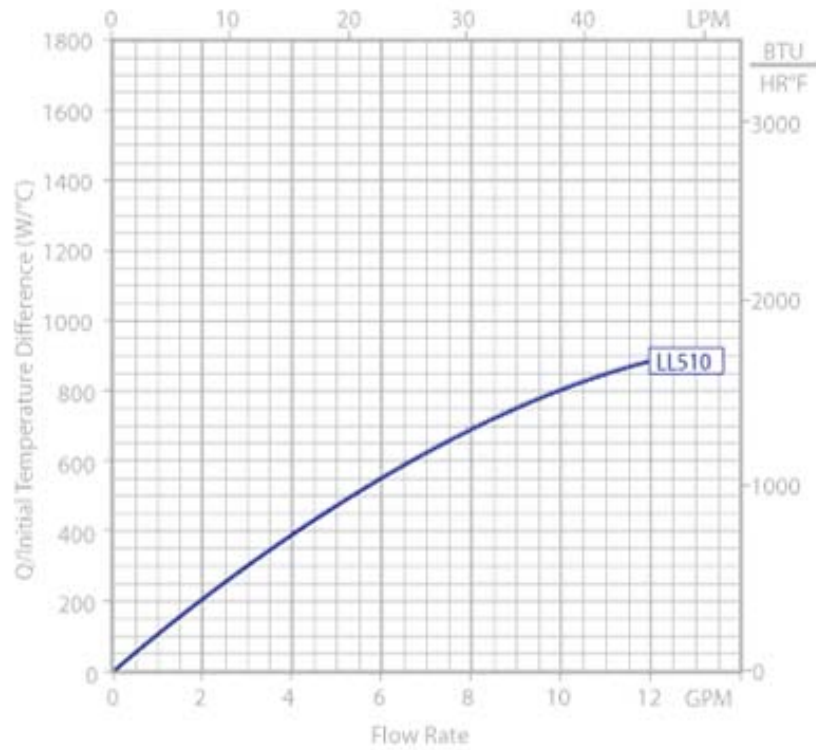
Liquid-to-Liquid Thermal Performance Using Water and Water
