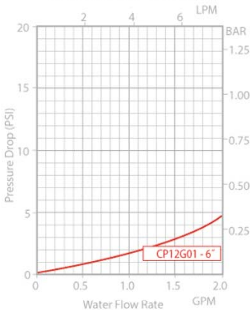
CP12G01 Pressure Drop
