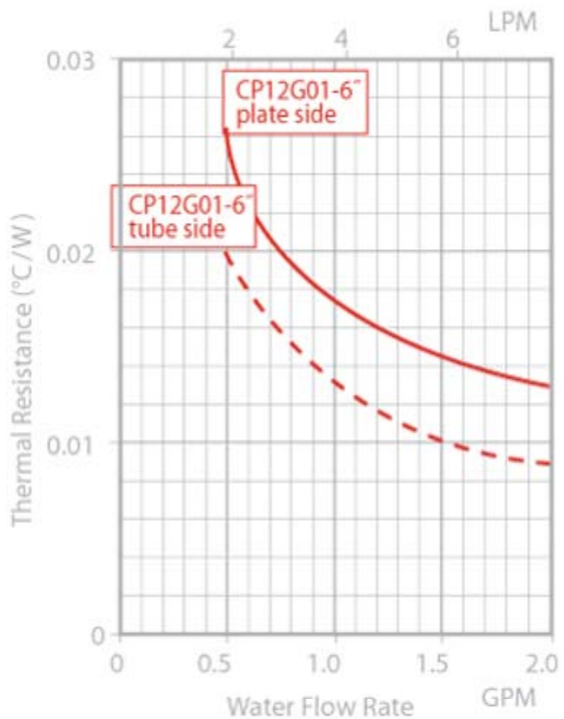
CP12G01 Thermal Resistance
