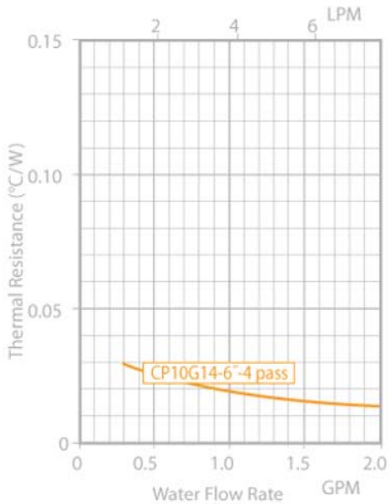
CP10G14 Thermal Resistance
