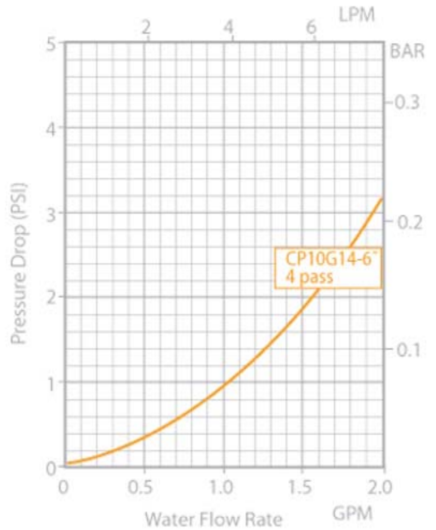
CP10G14 Pressure Drop
