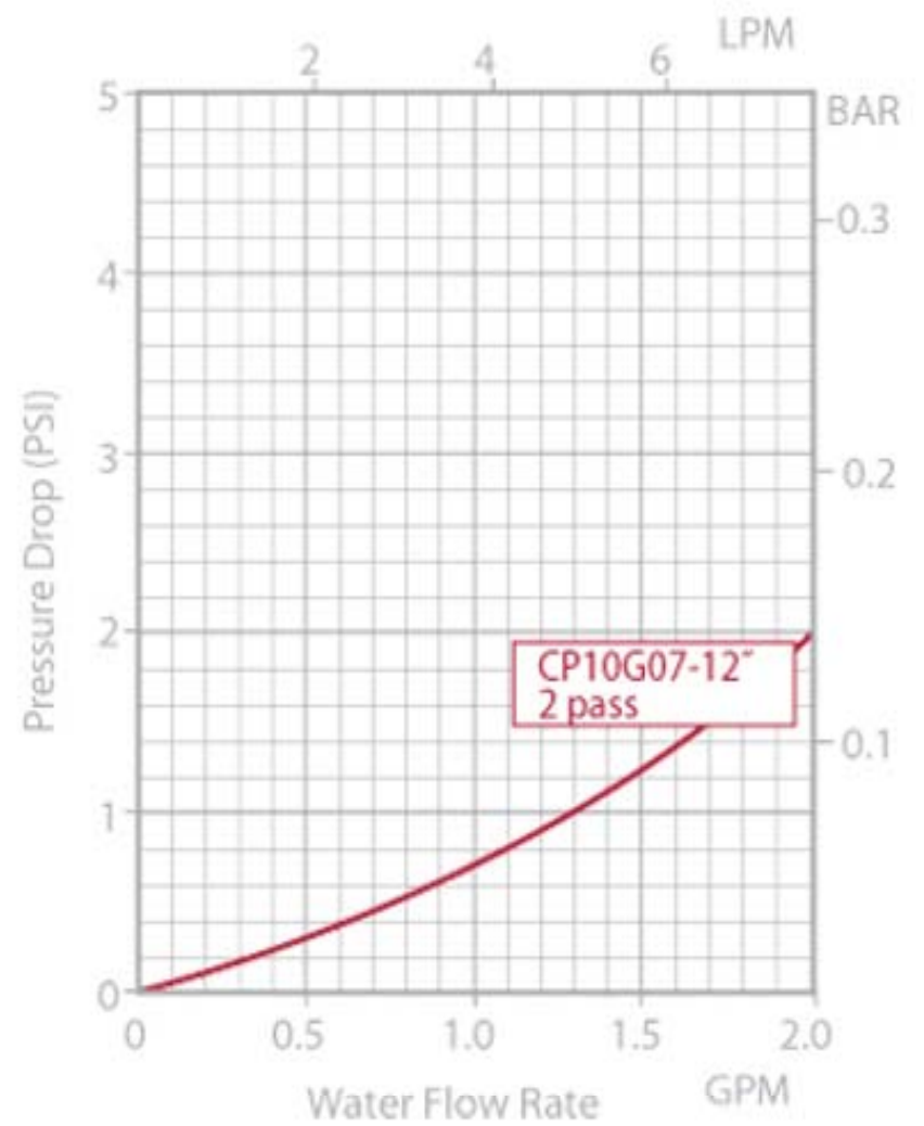
CP10G07 Pressure Drop
