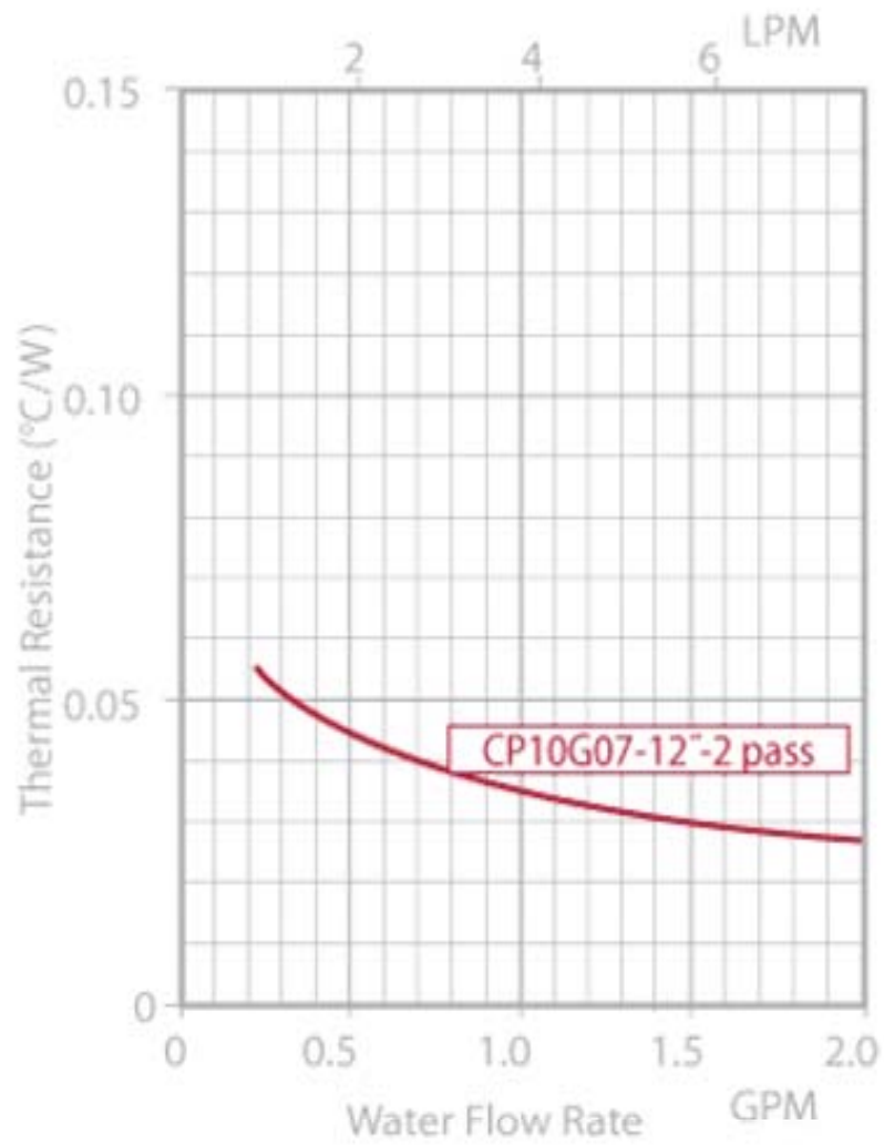
CP10G07 Thermal Resistance
