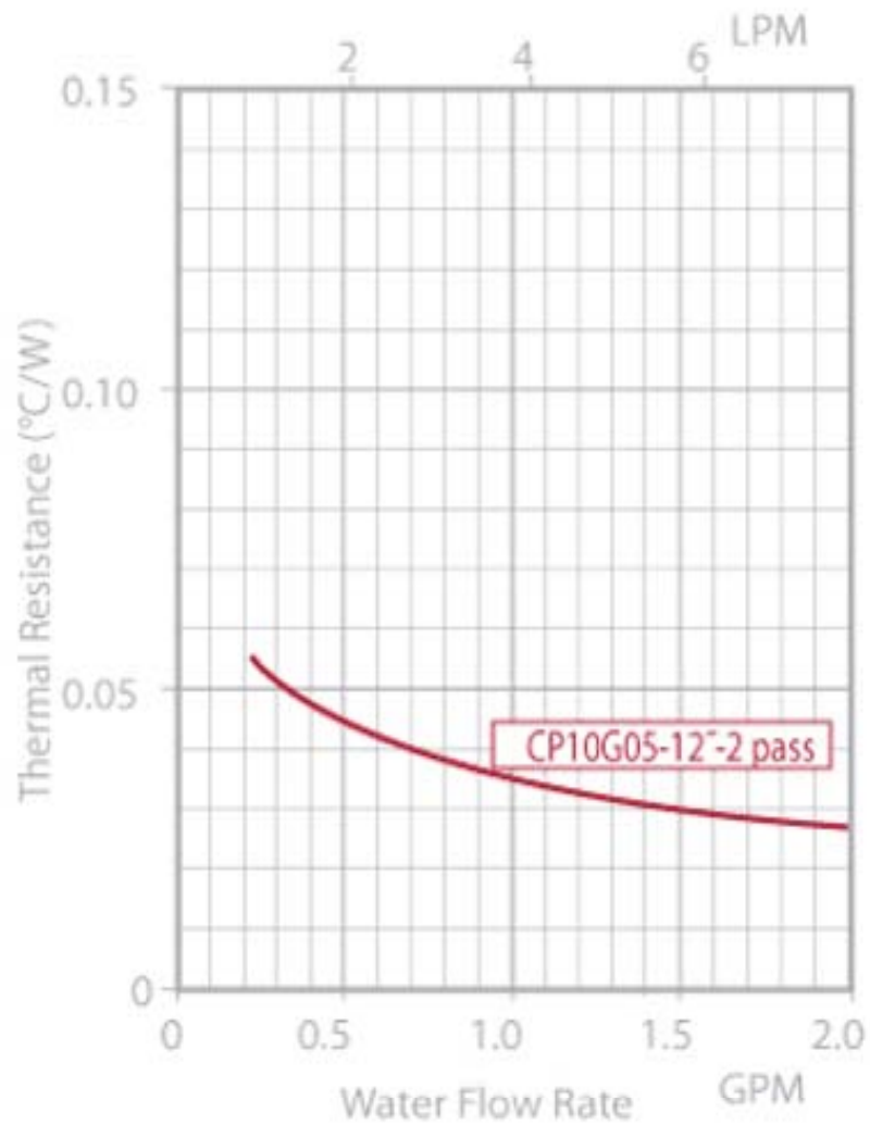
CP10G05 Thermal Resistance
