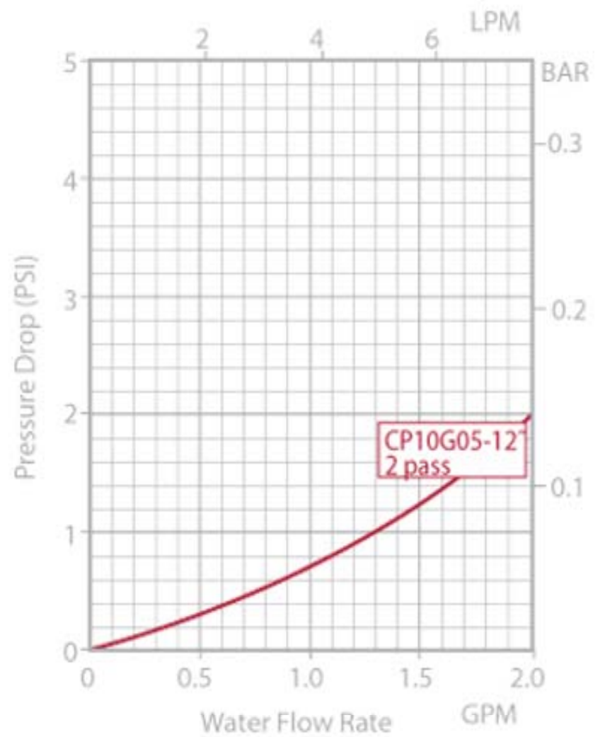
CP10G05 Pressure Drop
