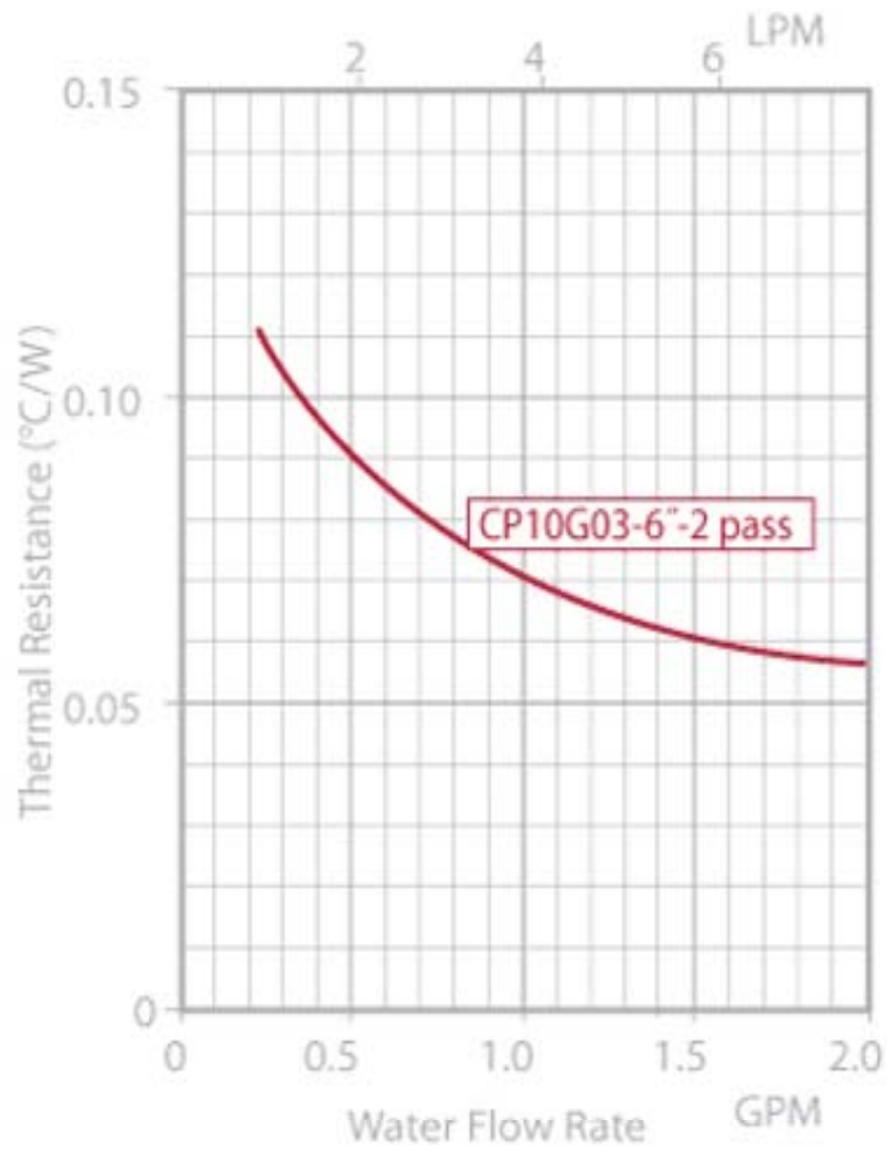
CP10G03 Thermal Resistance
