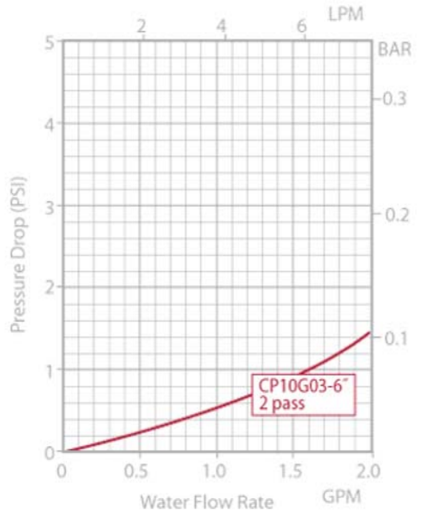
CP10G03 Pressure Drop
